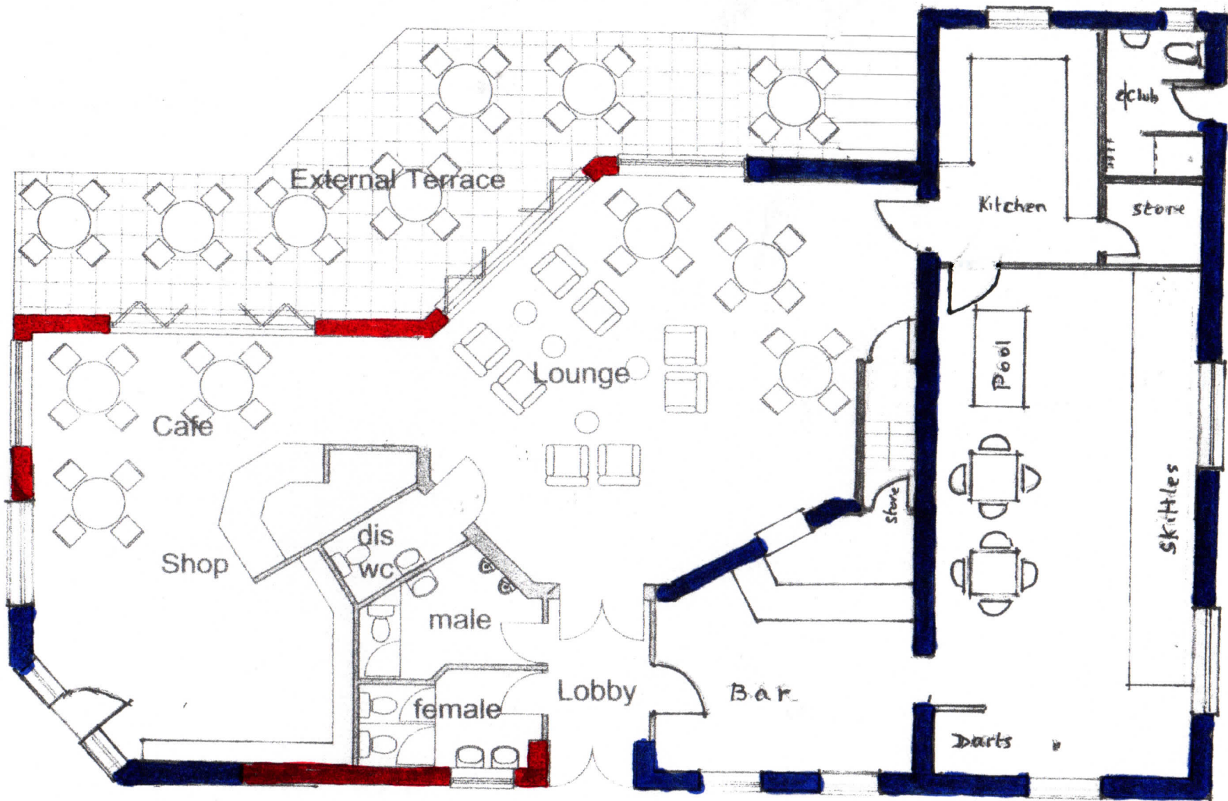
Ground Floor Plan 1:100 at A3
